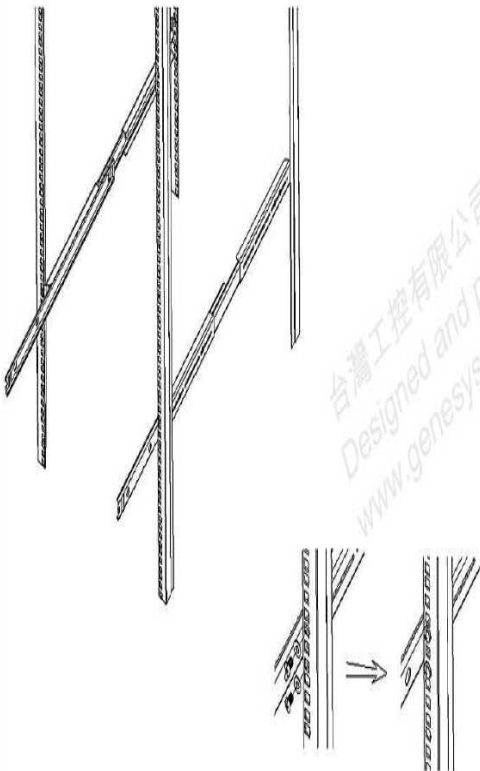
Stage4: Outer rail installed with cabinet in advance
