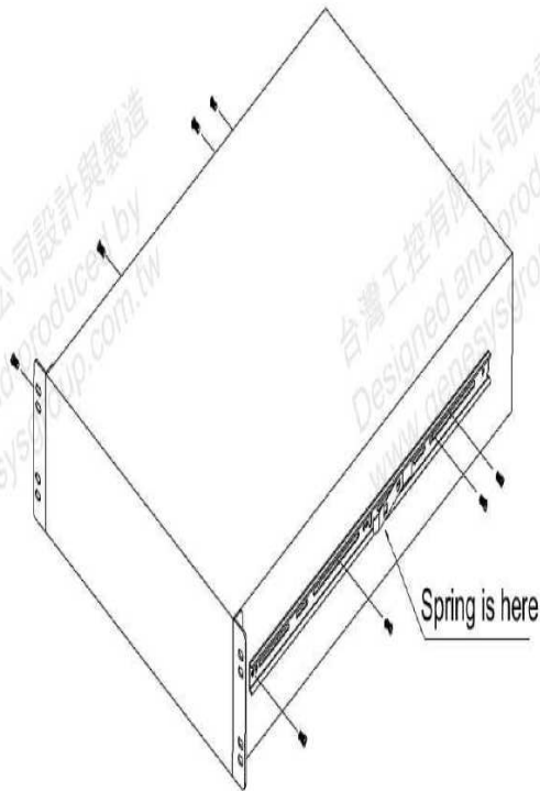
Stage2: Install the inner rail with two sides of chassis first
