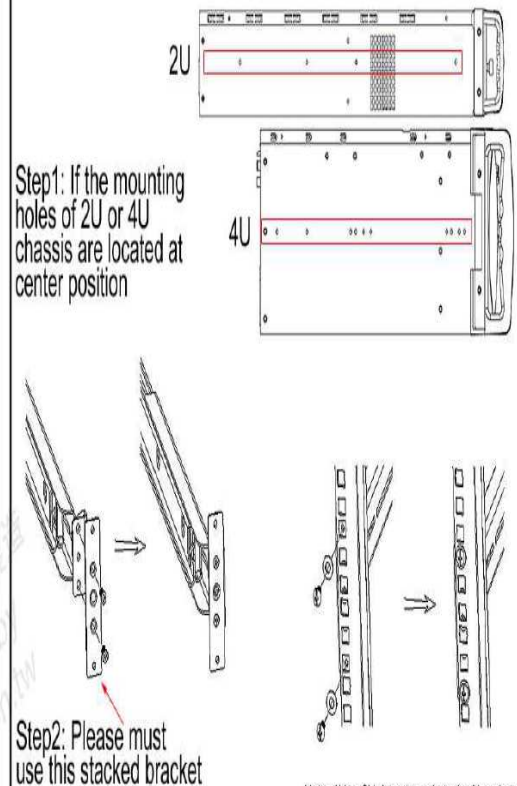
Stage6: Stacked brackets (standard part) for some 2U/4U cases
