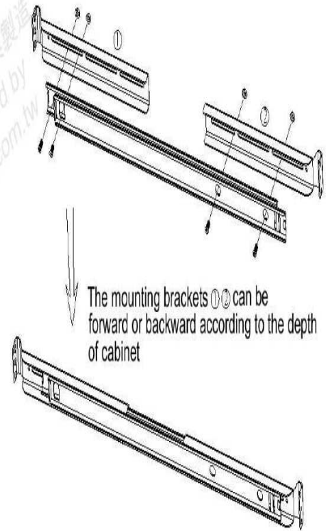
Stage3: Outer rail assembly
