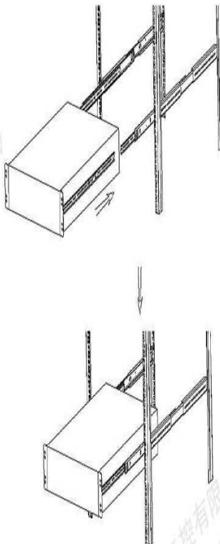
Stage5: Push in the chassis (inner rail installed) to the cabinet
